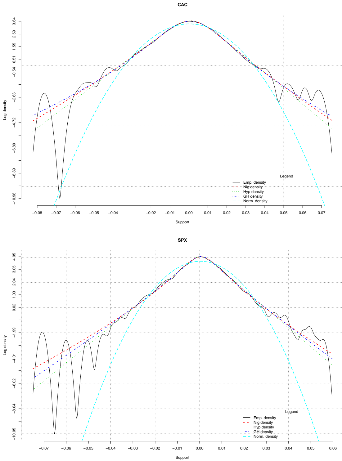
Figure 1: Log-density
