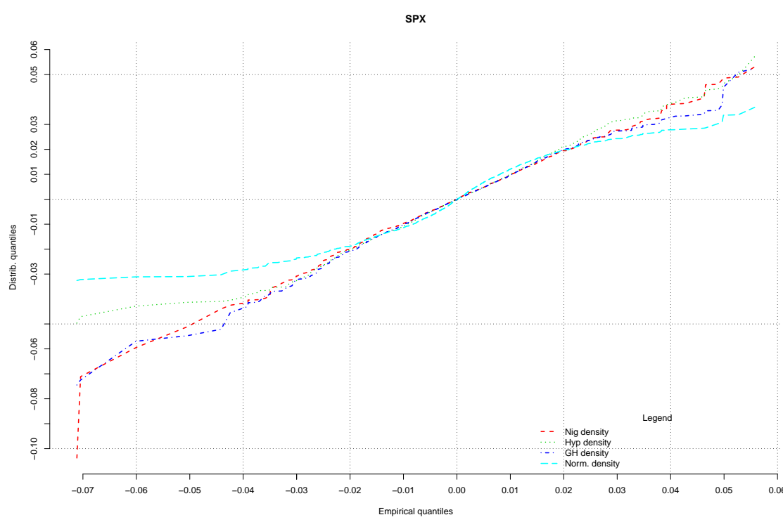
Figure 2: QQ-Plot
