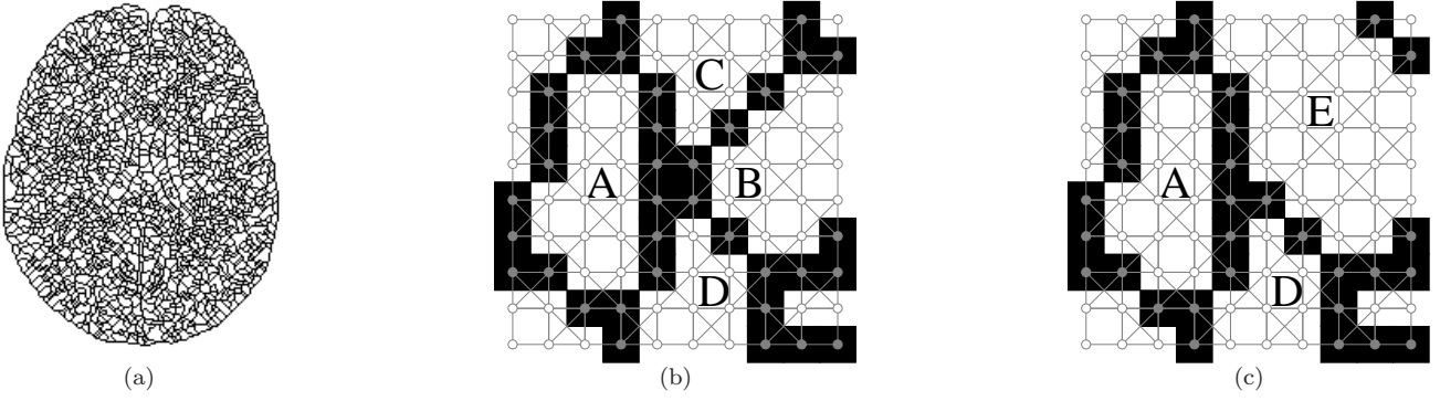
Fig. 3 (a) A segmentation of Fig. 1a obtained on a perfect fusion grid. (b) A zoom on a part of (a); the regions A, B, C and D correspond to the ones of Fig. 1c; the corresponding perfect fusion grid is shown in gray. (c) Same as (b) after having merged B and C to form a new region E.
