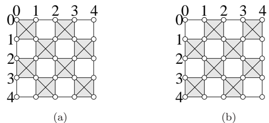
Fig. 2 Illustration of the two perfect fusion grids on \mathbb{Z}^2 . The gray squares constitute subsets of the two chessboard on \mathbb{Z}^2 and the associated graphs are the subgraphs of the perfect fusion grids (\mathbb{Z}^2, \mathcal{A}_{(1,1)}^2) and (\mathbb{Z}^2, \mathcal{A}_{(1,0)}^2) induced by \{0, \dots, 4\} \times \{0, \dots, 4\} .
