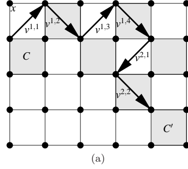
Fig. 12 Illustration of the method used to prove Lemma 17. We suppose that \mathbb{Z}^2 is oriented as shown in Fig. 9 and that x = (0, 0) and we consider C and C' as the 2-cubes of \mathcal{C}_{(0,1)}^2 defined by \varphi(C) = (0, 1) and \varphi(C') = (4, 3) .
