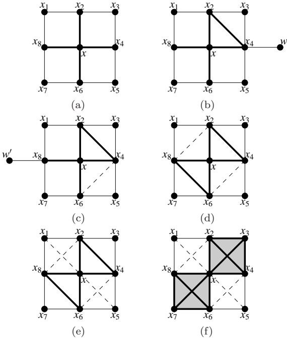
Fig. 13 Configurations used to prove Theorem 21 when the dimension d equals 2 [see text]. In each sub-figure the bold (resp dashed) edges indicate the edges which belong (resp. do not belong) to the perfect fusion graph \Gamma^2 .
