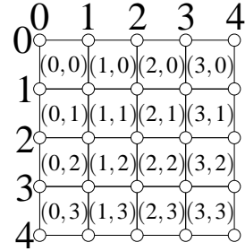
Fig. 8 Index map of \mathcal{C}^2 associated with a subset of \mathbb{Z}^2 .
