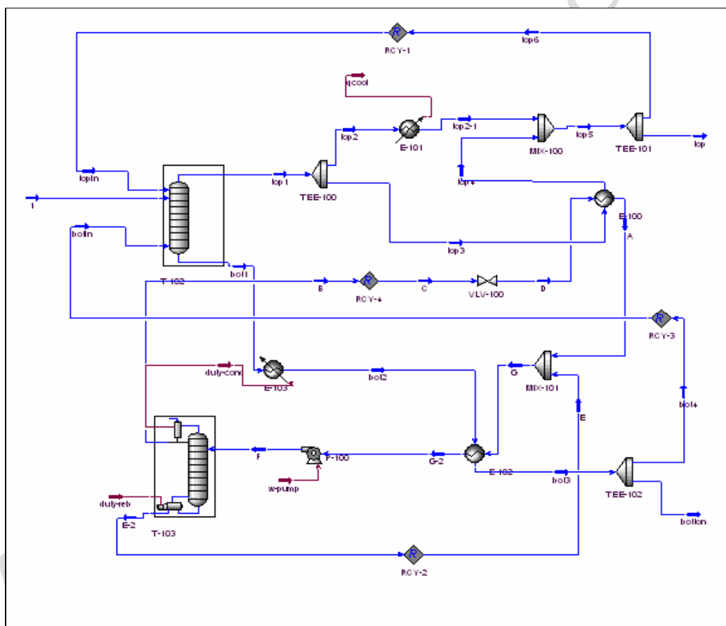
Figure 4: HYSYS Process Flow diagram for the absorption heat pump
