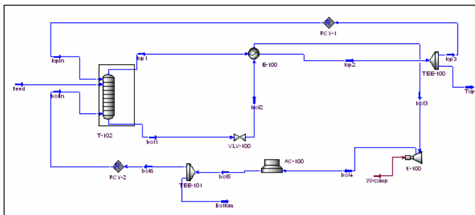
Figure 3: HYSYS Process Flow diagram for the bottom flashing heat pump
