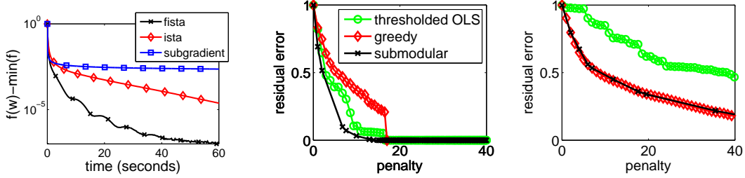
Figure 4: (Left) Comparison of iterative optimization algorithms (value of objective function vs. running time). (Middle/Right) Relaxation of combinatorial optimization problem, showing residual error \frac{1}{n}\|y - X\hat{w}\|_2^2 vs. penalty F(\text{Supp}(\hat{w})) : (middle) high-dimensional case ( p = 120, n = 20, k = 40 ), (right) lower-dimensional case ( p = 120, n = 120, k = 40 ).
