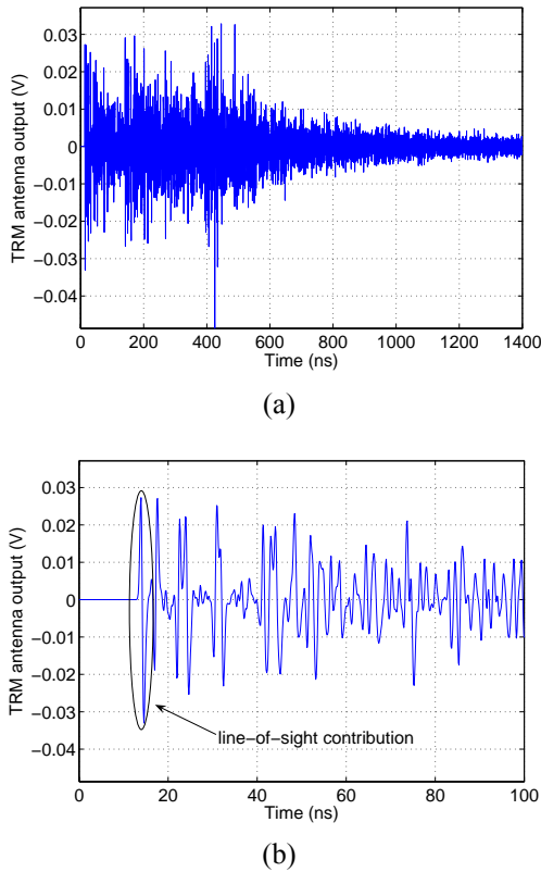
Figure 4 - Time-domain signals received by a TRM probe: (a) the typical decay of RCs, setting the minimum time needed for each measurement and (b) a zoom over the early-time response, showing the negligible impact of the line-of-sight contribution (first doublet).
