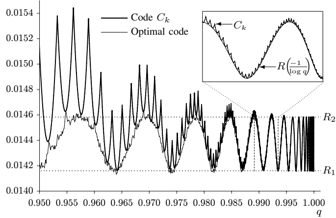
Fig. 8. Redundancy as q \rightarrow 1 ( k \rightarrow \infty ). Dashed lines show the asymptotic limits R_1 and R_2 . The inset closes up further on a narrow segment, showing the redundancy of the codes C_k vs. the asymptotic estimate (43).
