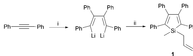
Scheme 1 Synthesis of 1-allyl-1-methyl-2,3,4,5-tetraphenylsilole ( 1 ). Reagents and conditions: (i) Li shavings, THF, 12 h and room temperature; (ii) allylmethylchlorosilane, THF, 2 h at room temperature and 5 h under reflux.
