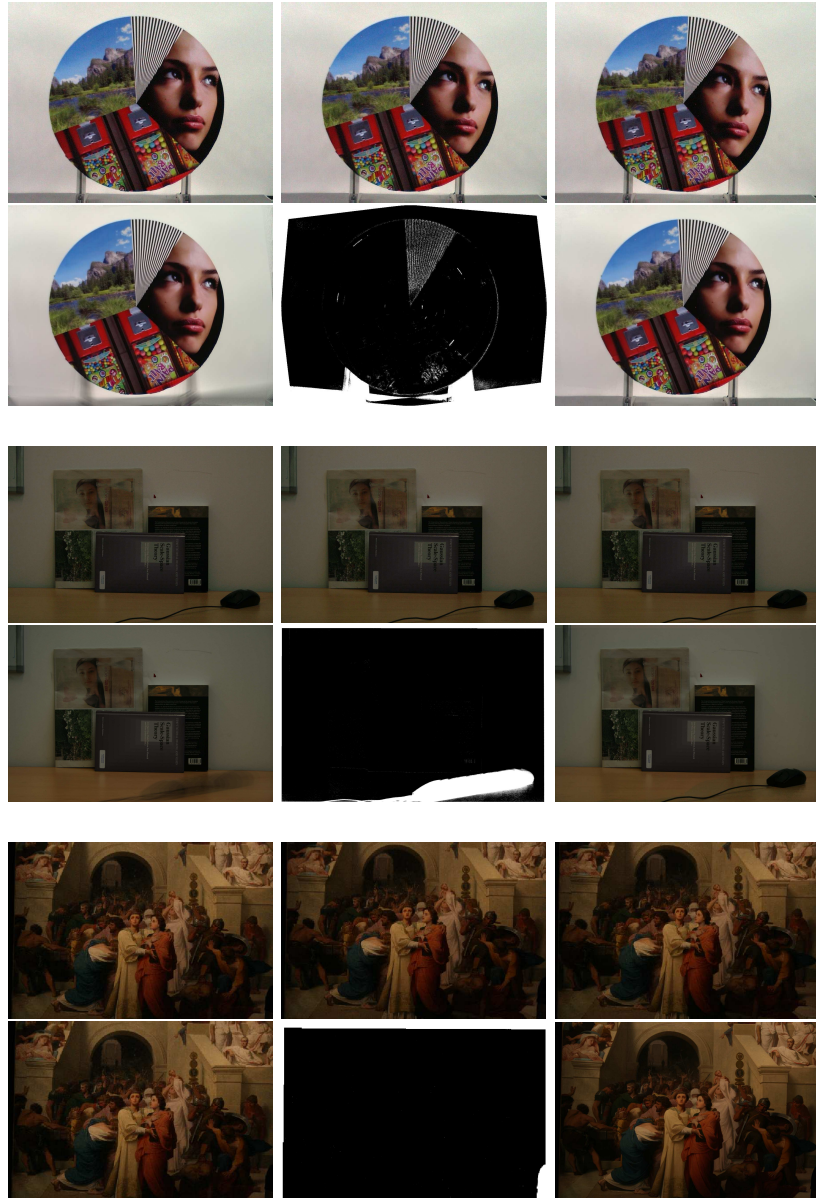
Figure 7: In each double row: three images of a sequence in the first row. In the second row on the left the average after registration, in the middle the mask of points with a too large temporal standard deviation, and on the right the restored image by hybrid method. These experiments illustrate how the hybrid method detects and corrects the potential wrong registrations due to local errors in the global homography.
