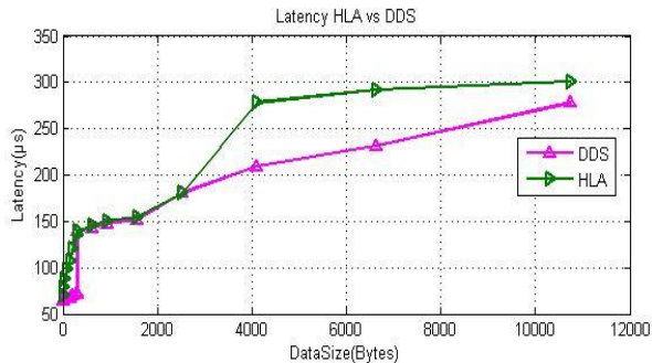
Figure 9: Point-to-point node Latency
