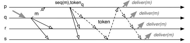
Fig. 2. The token-passing mechanism with Uniform delivery
