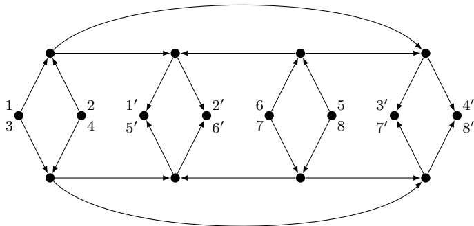
Figure 1: Example of a planar acyclic instance with r + c Eulerian, where there is a half-integral solution, but no integral solution.
