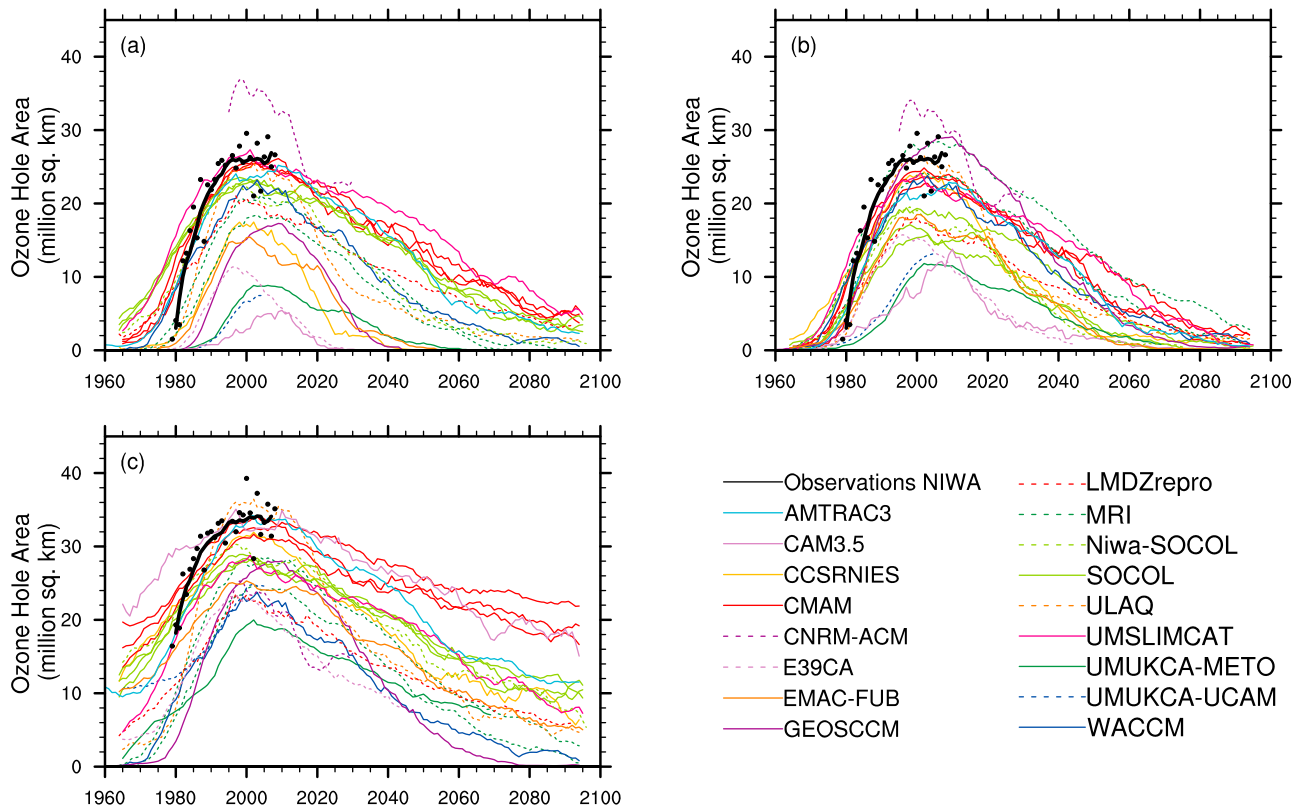
Figure 4. Simulated and observed ozone hole areas, (a) based on a fixed, 220 DU amount, (b) based on the 1960–1965 minimum, and (c) based on the value at the maximum gradient. The curves indicate 11 year running means of the observations and model results for individual years. The model results have been obtained from the REF-B2 simulations.
