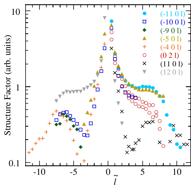
Fig. 2. Experimental structure factors of crystal truncation rods on Au(332), as a function of
