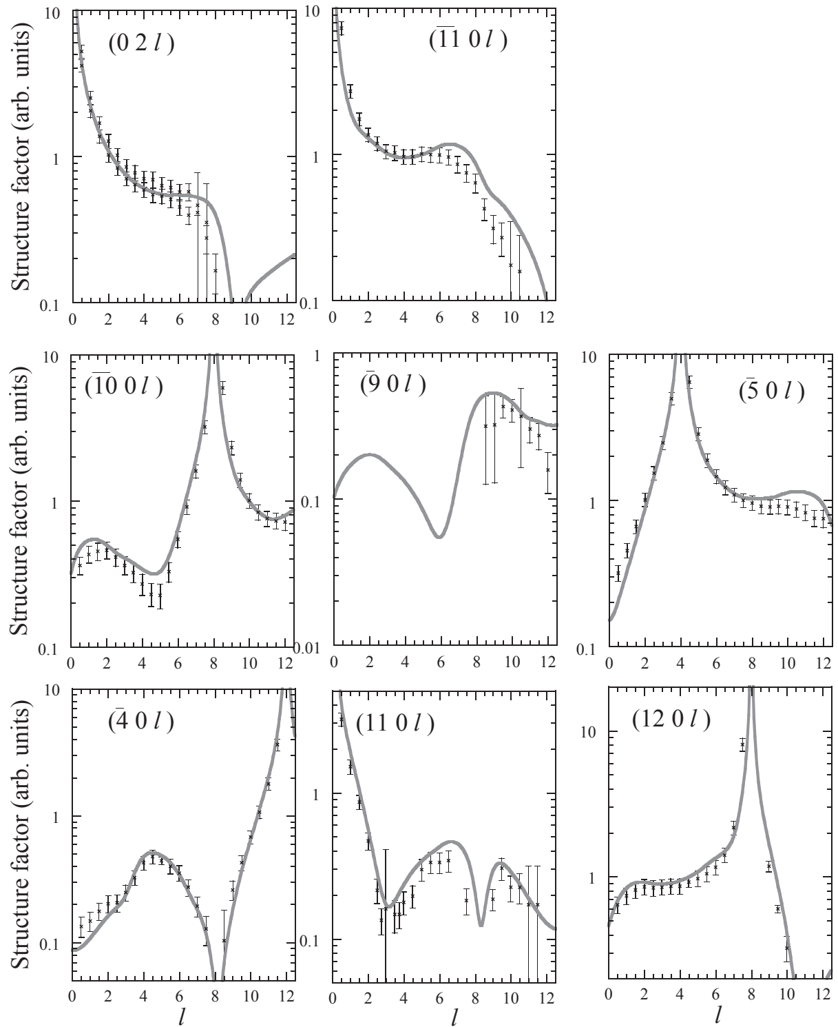
Fig. 5. Comparison between experimental and theoretical structure factors for Au(332). The dots are the experimental data, while the lines are the values calculated making use of the ab initio DFT results for atomic relaxations.
