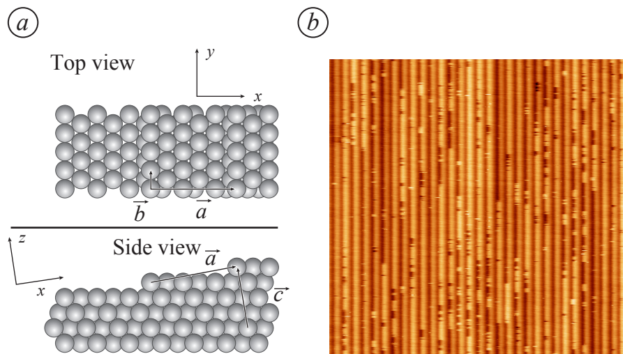
Fig. 1. (a) Schematic diagram of the atomic arrangement on the Au(332) surface, including the unit cell (\vec{a}, \vec{b}, \vec{c}) for GIXD measurements, and (b) 40 nm STM image of the Au(332) surface.
