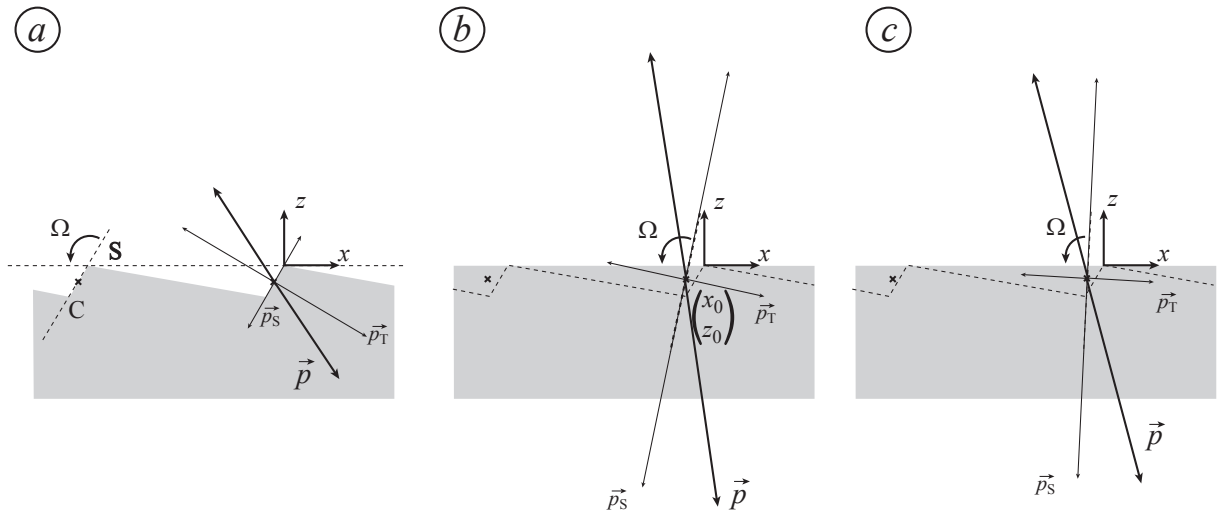
Fig. 4. Schematic diagrams showing the dipolar distributions given in Table 1. (a) point dipole equivalent to the initial force distribution on the step edge (S) and corner (C) atoms computed by DFT for a bulk-truncated slab, (b) elastic point dipole giving the same displacements as the atomic relaxations computed by DFT, and (c) elastic point dipole that gives the best fit to the GIXD results. \Omega is the orientation of the lever arm of the dipole with respect to the surface, and x_0 and z_0 are the position of the dipole with respect to the step edge. The dipole is the sum of a torque component \vec{p}_T and a stretch component \vec{p}_S . Note that the (b) and (c) distributions are very similar.
