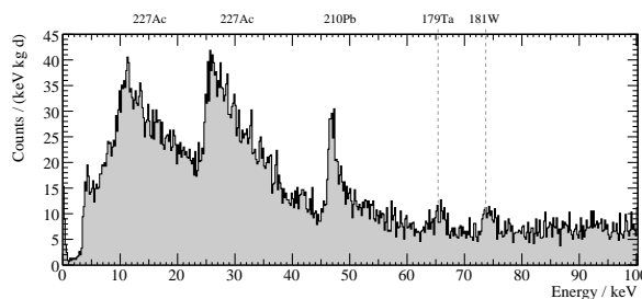
Figure 6: Background spectrum recorded in 2007 from a third detector ( m = 307.0\text{ g} ) with an exposure of 22.81 kg d (detector ZORA, run 30).
