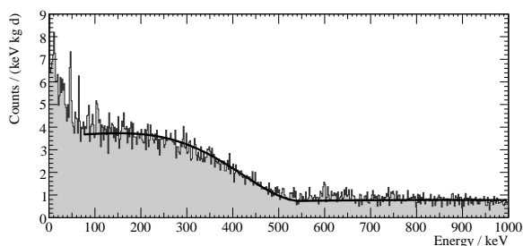
Figure 3: Background spectrum observed with one crystal ( m = 306.8\text{ g} ) from an exposure to background radiation of 15.00 kg d early 2004 (detector DAISY, run 28). The black line is a fit above 80 keV of a parametrization of the ^{90}\text{Sr}/^{90}\text{Y} beta spectrum to the data.
