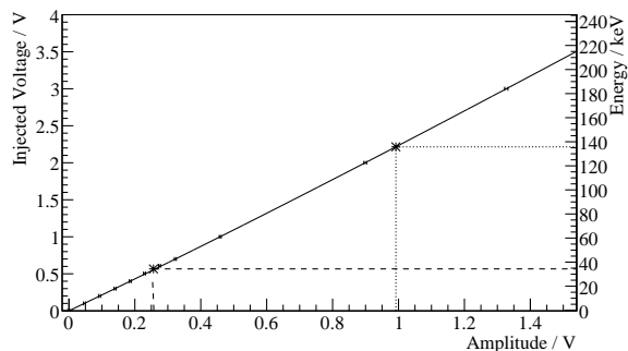
Figure 1: Calibration at low energies with heater pulses of various discrete energies. Fitting a low order polynomial to the thermometer response (small points, including error bars) gives the transfer function (solid line) between injected voltage (scale on the left) and fitted amplitude (scale on the bottom). The 136 keV peak gives a calibration point (dotted line) for the injected energy (scale on the right). Then, for each particle pulse, the particle's energy is found by evaluating the transfer function at the fitted amplitude (dashed line).
