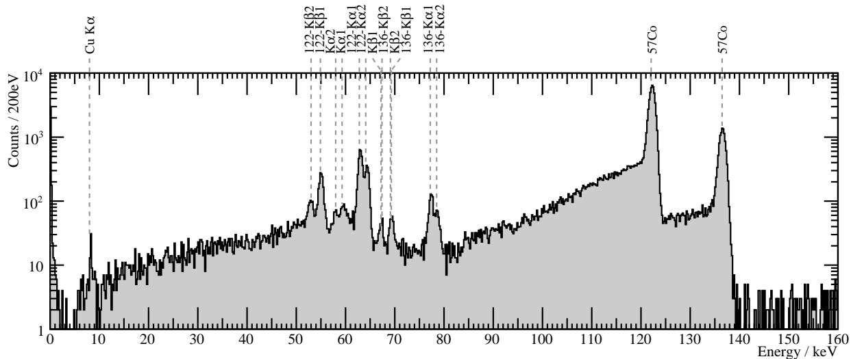
Figure 2: Energy spectrum from a high statistics ^{57}\text{Co} calibration (detector DAISY, run 31). The relative strengths of escape peaks to direct gamma lines depend on the position of the crystal, the source, as well as the position of neighbouring crystals and the surrounding cryostat and is in agreement with simulations.
