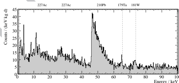
Figure 5: Background spectrum of a second crystal ( m = 305.5\text{ g} ) from an exposure of 21.20 kg d in 2007 (detector VERENA, run 30).
