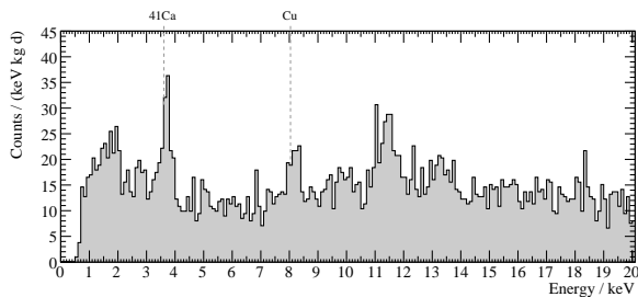
Figure 8: Low-energy part of the spectrum shown in figure 5. In addition to the lines from ^{41}\text{Ca} and copper fluorescence there is a line at \sim 11.5 keV which so far could not be identified in a consistent way (detector VERENA, run 30).
