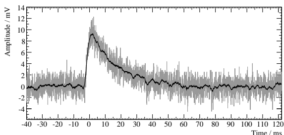
Figure 9: A typical pulse with an energy of 3.7 keV (grey), and its 50-sample (2 ms) moving average (black).
