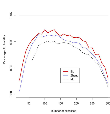
(d) Coverage Probability for Frchet(1/4) model, n = 1000
