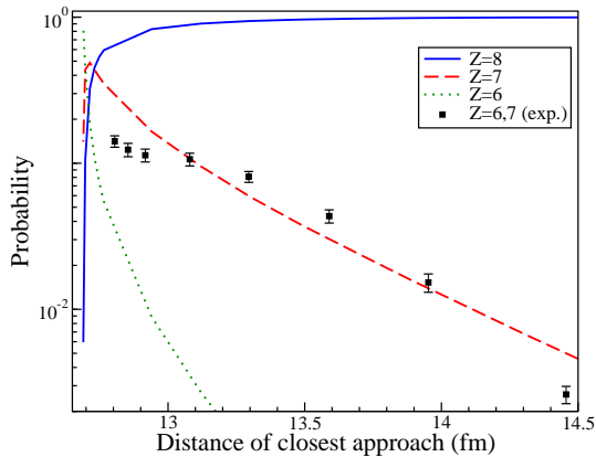
FIG. 3: Proton number probability distribution as function of the distance of closest approach obtained with TDHF (lines). Experimental data (squares) are adapted from Ref. [26] using E_{c.m.} = 74.3 MeV data and show the sum of the one and two-proton transfer channels.
