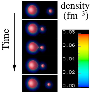
FIG. 1: (color online) Density evolution for the central collision of a ^{16}\text{O} (initially on the right side) with a ^{208}\text{Pb} (left) at E_{c.m.} = 74.44 MeV. The snapshots run from t = 7.5 to 37.5 zs by steps of 7.5 zs.
