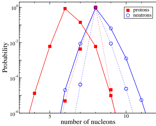
FIG. 2: Neutron (circles) and proton (squares) number probability distributions of the lightest fragment in exit channel of a head-on ^{16}\text{O}+^{208}\text{Pb} collision at E_{c.m.} = 74.44 MeV (solid lines) and 65 MeV (dotted lines).
