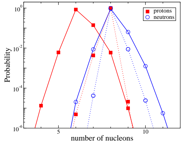
FIG. 2: Neutron (circles) and proton (squares) number probability distributions of the lightest fragment in exit channel of a head-on ^{16}\text{O} + ^{208}\text{Pb} collision at E_{c.m.} = 74.44 MeV (solid lines) and 65 MeV (dotted lines).
