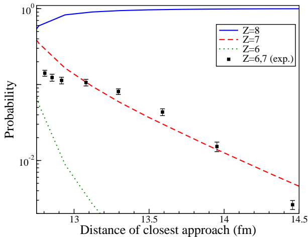
FIG. 3: Proton number probability distribution as function of the distance of closest approach obtained with TDHF (lines). Experimental data (squares) are adapted from Ref. [27] using E_{c.m.} = 74.3 MeV data and show the sum of the one and two-proton transfer channels.
