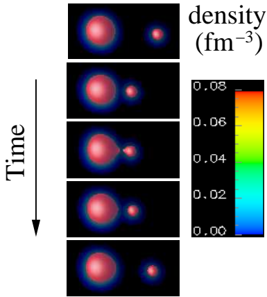
FIG. 1: (color online) Density evolution for the central collision of a ^{16}\text{O} (initially on the right side) with a ^{208}\text{Pb} (left) at E_{c.m.} = 74.44 MeV. The snapshots run from t = 7.5 to 37.5 zs by steps of 7.5 zs.
