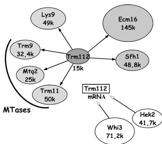
FIGURE 6. Partners of Trm112p. The figure schematically represents six putative partners of Trm112p. The four proteins represented in light shading correspond to the ones that were predicted to be Trm112p partners when we initiated this study (10, 34) and that were then confirmed individually by co-immunoprecipitation. They all possess a Rossman fold domain that is the signature of enzymes utilizing S-adenosylmethionine as a co-factor, and they are all confirmed MTases, except for Lys9p, which lacks one of the seven β-strands of the fold. The proteins shown in darker shading were reported more recently and do not possess a Rossman fold. Ecm16/Dhr1p was shown to interact with Trm112p in a recent proteomic analysis (52). It is a DEAH-box ATP-dependent RNA helicase involved in rRNA maturation (53). Sfh1p was then reported to interact with Trm112p in a two-hybrid interactome network (36). It is a component of the RSC complex that is phosphorylated during the G 1 phase of the cell cycle. It is encoded by an essential gene, and the protein is required for cell cycle progression and maintenance of proper ploidy (37, 38). Two more proteins are represented on a white background, with arrows pointing to TRM112 mRNA. Hek2/Khd1p and Whi3p are RNA-binding proteins that were found to participate in the localization of numerous mRNA at the tip of the bud (54) and at the endoplasmic reticulum (55), respectively.
