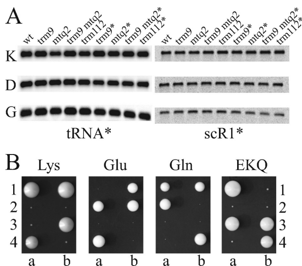
FIGURE 5. tRNA steady-state levels in different mutants. A , total RNA was separated on denaturing 1.2% agarose gel, transferred under vacuum to charged nylon membrane, and probed as indicated. K , D , and G , probes for tRNA Lys, Glu, and Gly, respectively. scR1 , the three membranes were re-probed with scR1 for normalization. The origin of each RNA sample is shown at the top; the five lanes on the left are from strains constructed in the W303 background, and the four lanes on the right, with asterisks, are in the S288c background. wt , wild type. B , a diploid strain heterozygous for the trm112-0 deletion was transformed with high copy number plasmids expressing tRNA Lys , tRNA Glu , tRNA Gln , or the three tRNA together ( EKG ), as indicated. These strains were then sporulated, the tetrads were dissected, and the growth of the resulting spores containing the plasmids was tested at 30 °C. Shown here are the results for two tetrads ( lanes a and b ) for each transformant. The large colonies (such as lane a , rows 1 and 4, and lane b , rows 1 and 3, for tRNA Lys , for instance) were tested and found to be wild type for TRM112 , whereas the small ones were trm112::kanMX4 . None of the tRNA expressing plasmids was able to compensate for the growth defect of the trm112-0 strain.
