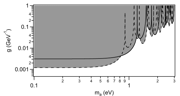
FIG. 2: 95 % confidence level limits on the ALP-two photon coupling constant g as a function of the particle mass m_a . The grey area is excluded. The dashed line represents limits obtained with a photon energy of 50.2 keV while the solid line corresponds to 90.7 keV.
