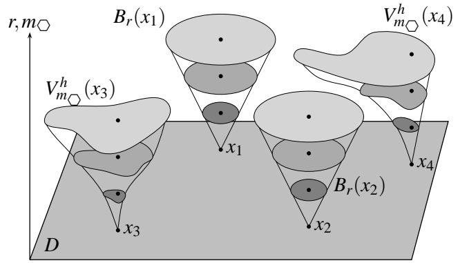
Fig. 2. Classical neighborhoods B_r(x) vs. general adaptive neighborhoods V_{m_\square}^h(x) .
