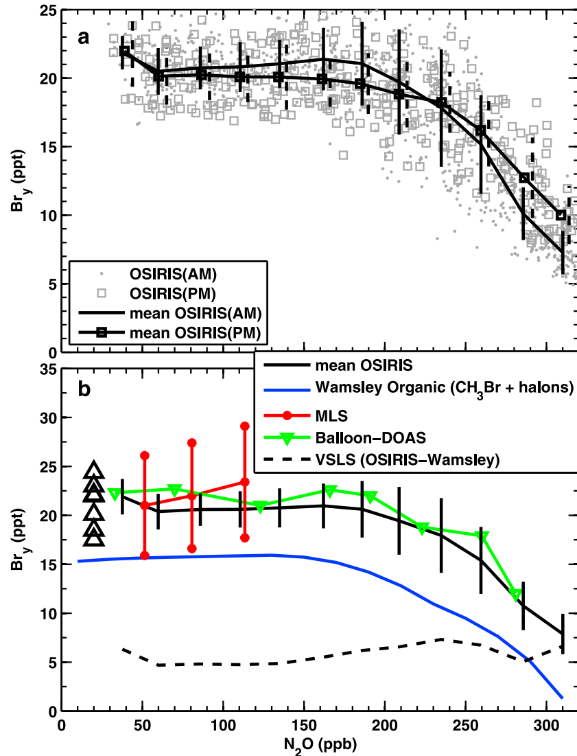
Figure 17. (a) Tracer correlation plot of OSIRIS Br_y and Odin/Submillimetre and Millimetre Radiometer N_2O monthly mean from 40^\circ S to 40^\circ N shown separately for AM and PM measurements. Each symbol represents an individual altitude/latitude. Lines represent mean Br_y averaged over 20 ppbv wide bins in N_2O and their 1\sigma standard deviation (shown dashed for PM values). (b) Tracer correlation of Br_y and N_2O for different data sources. The open triangles represent inferred total Br_y from other studies (without accompanying N_2O ). MLS, Microwave Limb Sounder.
