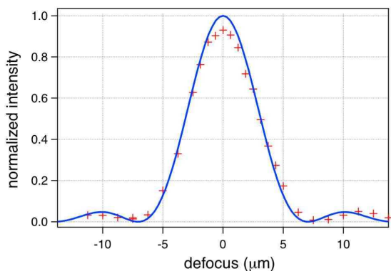
FIG. 4: (Color Online) On-axis intensity variation close to the focal point, as a function of the position along the optical axis. The prediction from diffraction theory is shown for comparison, with the intensity normalized as in Fig. 2.
