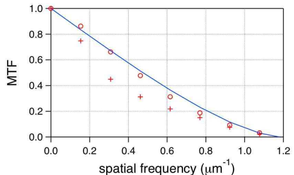
FIG. 5: (Color Online) Modulation transfer function (MTF) of the tweezer system. MTF measured on-axis (circles) and off-axis by 30 \mu\text{m} (crosses) are compared to the theoretical frequency response of an aberration-free system (solid line). Strehl ratio is S = 0.93 on-axis, and S = 0.77 off-axis.
