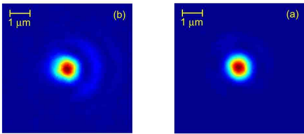
FIG. 3: (Color Online) Images of the point spread function of our tweezer system, taken with a linear CCD camera at 850 nm, for a sub-micron pinhole source on axis (a) and off-axis by 30 \mu\text{m} (b). Cross-sections shown on Fig. 2 were taken along the horizontal axis of these images, across the center, where intensity is maximum.
