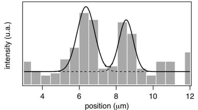
FIG. 7: Cross-section of a CCD image showing two single atoms trapped in two adjacent optical tweezers, corrected for the magnification ( \times 25 ) of the imaging system. The distance between the two optical tweezers is 2.2 \pm 0.1 \mu\text{m} . Each peak is fitted by a gaussian model (dashed lines) and exhibits a waist w = 0.9 \pm 0.2 \mu\text{m} . The solid line represents the sum of the fits of the two fluorescence signals emitted by each single atom. Vertical bars represent the intensity measured by each pixel of the CCD camera during a time window of 100 ms.
