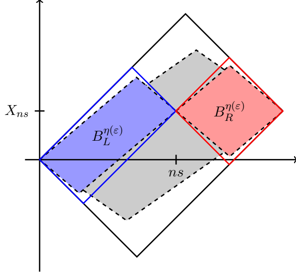
Figure 5: The \varepsilon -interiors B^\varepsilon (grey), B_L^{\eta(\varepsilon)} (blue) and B_R^{\eta(\varepsilon)} (red).
