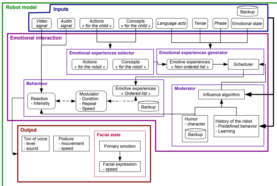
Fig. 2. Computal interaction model – iGrace
