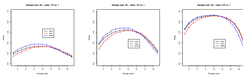
Fig. 2 Parametric test: power comparisons of the three tests for three alternatives
