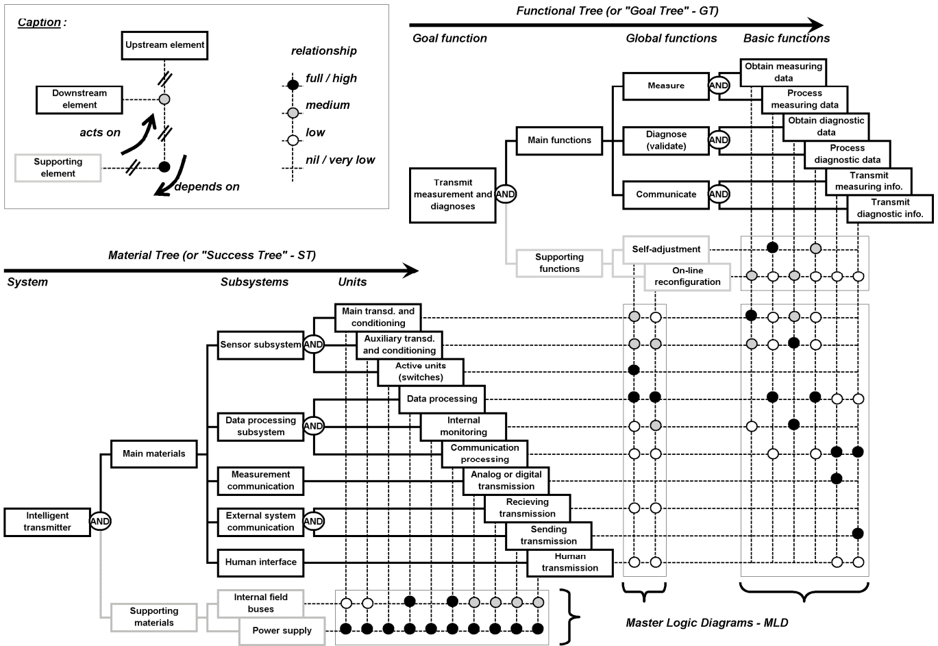
Fig 2. Reliability model proposal for an intelligent transmitter pattern
