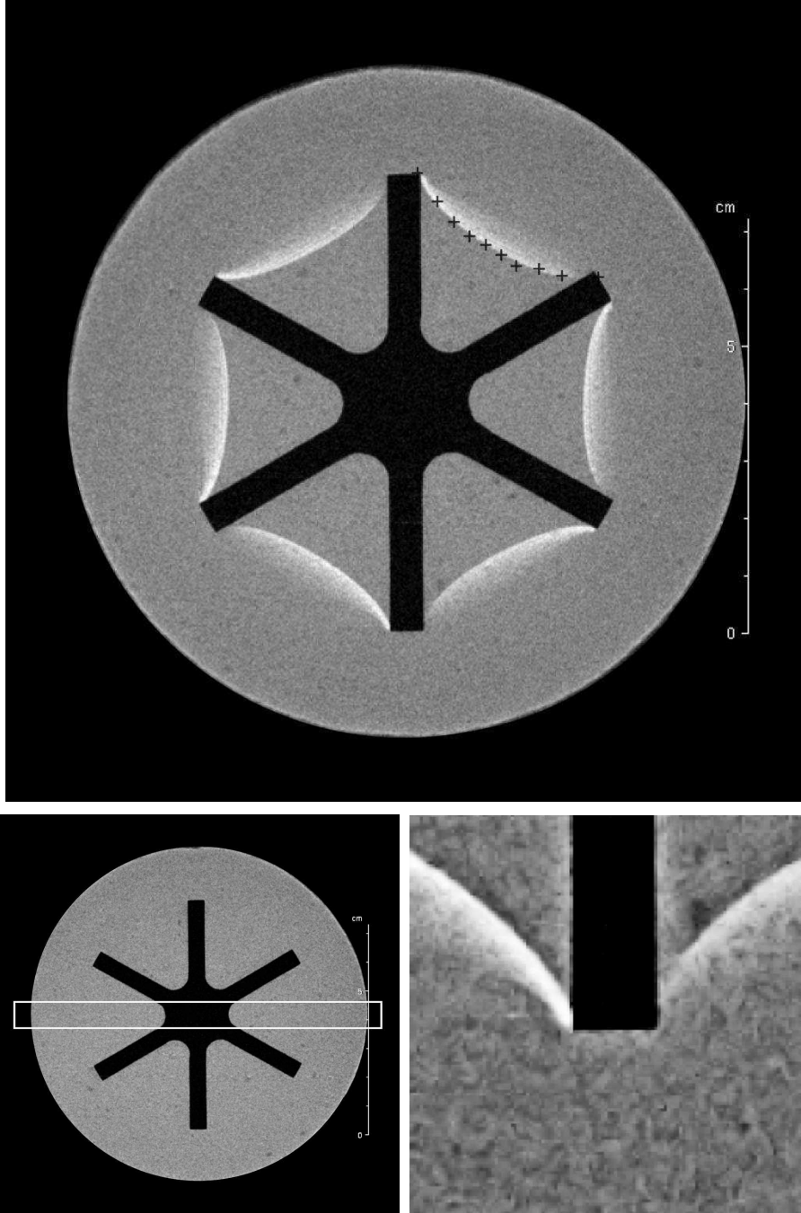
Figure 10: 2D magnetic resonance image of a suspension of particles in a yield stress fluid in a vane-in-cup geometry: (a) after a 1h shear at \Omega = 100 rpm (corresponding to a macroscopic strain of order 75000), and (b) before any shear. The crosses in Fig. 10a correspond to the limit between rigid motion and shear for the Newtonian oil of Fig. 3b. The white rectangle in Fig. 10b shows the slice in which the volume fraction profiles of Figs. 9a and 11 are performed. (c) is a zoom of image (a) near the edges of a blade. The images are taken in the horizontal plane of the geometry, at middle height of the vane tool, and correspond to vertical averages over 2 cm. The vane tool rotates counterclockwise.
