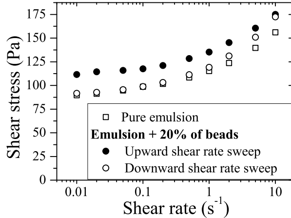
Figure 13: Shear stress vs. shear rate for upward/downward shear rate sweeps in a pure dense emulsion (open squares) and for the same emulsion filled with 20% of 140 \mu\text{m} PS beads (filled/open circles). Figure from Mahaut et al. (2008a).
