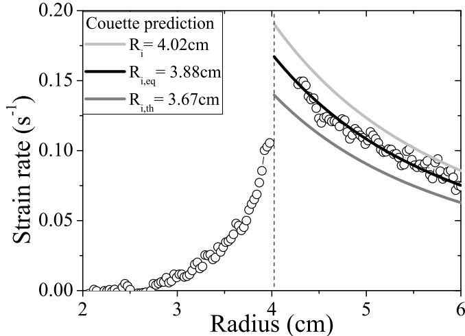
Figure 2: \theta -averaged strain rate \bar{d}_{r\theta} vs. radius r for a Newtonian oil sheared at 1 rpm in a 6-bladed vane-in-cup geometry. The dashed line shows the radius of the blades. The solid lines are the theoretical strain rate profiles for a Newtonian fluid in Couette geometries of radii: (i) R_i = 4.02 cm (light grey), (ii) R_{i,eq} = 3.88 cm (black), and (iii) R_{i,th} = 3.67 cm (dark grey) corresponding to the Atkinson and Sherwood (1992) theory in a infinite medium.
