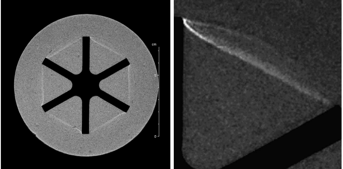
Figure 12: 2D magnetic resonance image of a suspension of particles in a yield stress fluid in the horizontal plane of a vane-in-cup geometry after a 14h shear at \Omega = 1 rpm (a). (b) is a zoom of image (a) between two adjacent blades. The image is taken in the horizontal plane of the geometry, at middle height of the vane tool, and corresponds to a vertical average over 2 cm. The vane tool rotates counterclockwise.
