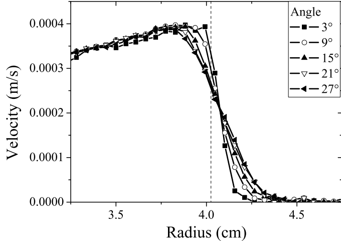
Figure 7: Orthoradial velocity profile V_\theta(r, \theta) of a yield stress fluid (dense emulsion) sheared at 0.1 rpm in a 6-bladed vane-in-cup geometry, for various angular positions \theta , from a blade ( \theta = 0^\circ ) to midway between adjacent blades ( \theta = 30^\circ ). The dashed line shows the radius of the blades.
