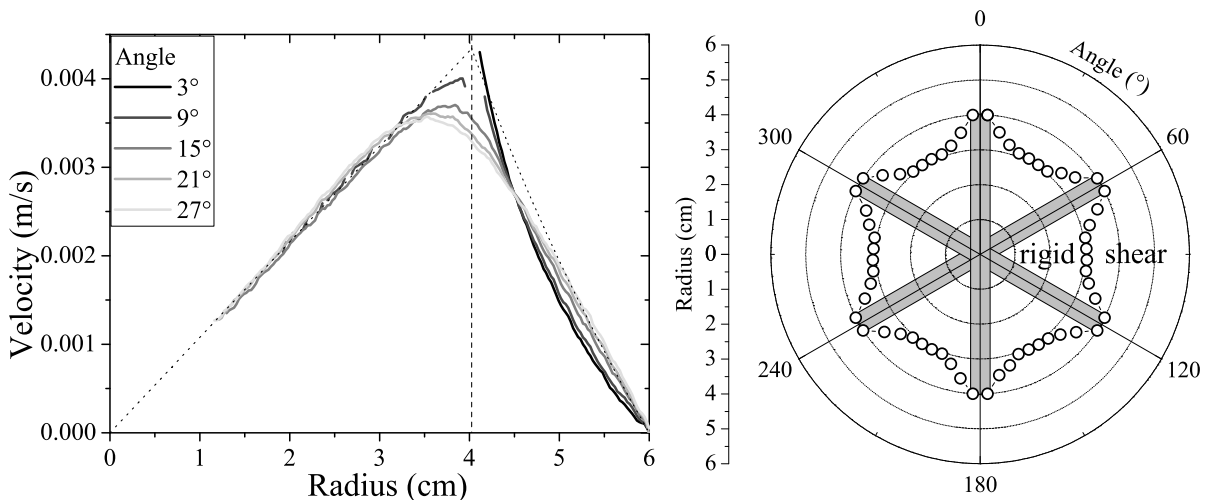
Figure 3: a) Orthoradial velocity profile V_\theta(r, \theta) of a Newtonian oil sheared at 1 rpm in a 6-bladed vane-in-cup geometry, for various angular positions \theta , from a blade ( \theta = 0^\circ ) to midway between adjacent blades ( \theta = 30^\circ ). The dashed line shows the radius of the blades. The dotted line is the profile for a rigid body rotation (for r < R_i ) and the theoretical profile for a Newtonian fluid in a Couette geometry of radius R_i (for r > R_i ). b) Two-dimensional plot of the limit between rigid motion and shear (empty circles) for a Newtonian material in the 6-bladed vane-in-cup geometry; the grey rectangles correspond to the blades.
