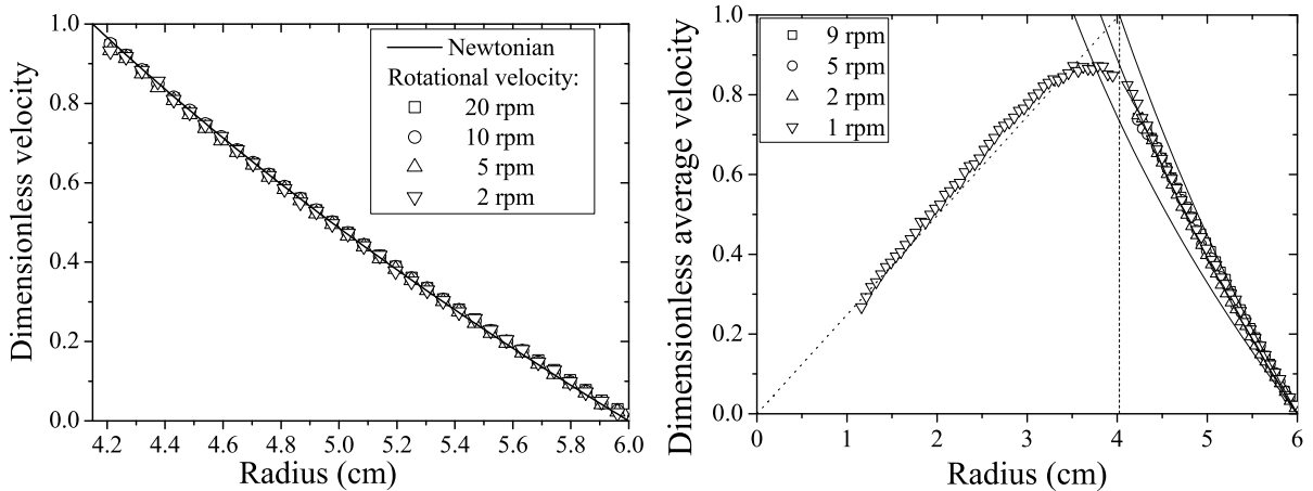
Figure 1: a) Dimensionless velocity profile V_\theta(r, \Omega)/\Omega R_i of a Newtonian oil in a Couette geometry ( R_i = 4.15 cm), at various rotational velocities \Omega ranging from 2 to 20 rpm; the solid line is the theoretical profile for a Newtonian fluid. b) Dimensionless \theta -averaged velocity profile \bar{V}_\theta(r, \Omega)/\Omega R_i of a Newtonian oil in a 6-bladed vane-in-cup geometry ( R_i = 4.02 cm) for \Omega ranging from 1 to 9 rpm; the dashed line shows the radius of the blades; the dotted line is the theoretical profile for a rigid body rotation (for r < R_i ); the solid lines are the theoretical profiles for a Newtonian fluid in Couette geometries of radii, from right to left: (i) R_i = 4.02 cm, (ii) R_{i,eq} = 3.88 cm, and (iii) R_{i,th} = 3.67 cm corresponding to the Atkinson and Sherwood (1992) theory.
