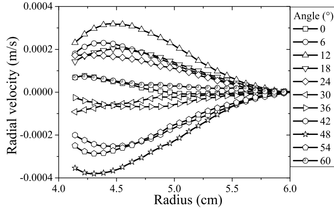
Figure 4: Radial velocity profile V_r(r, \theta) of a Newtonian oil sheared at 1 rpm in a 6-bladed vane-in-cup geometry, for various angular positions \theta between two adjacent blades (from \theta = 0^\circ to \theta = 60^\circ ).
