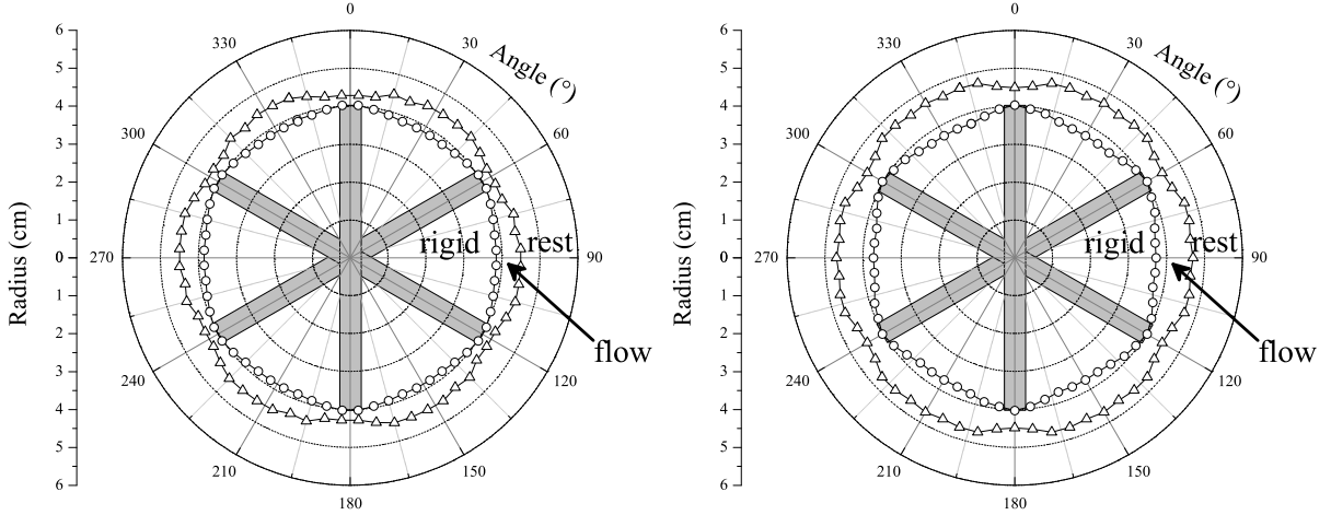
Figure 8: Two-dimensional plot of the limit between rigid motion and shear (circles) and between shear and rest (triangles) for a yield stress fluid (dense emulsion) sheared in the 6-bladed vane-in-cup geometry at 0.1 rpm (left) and 1 rpm (right). The grey rectangles correspond to the blades.
