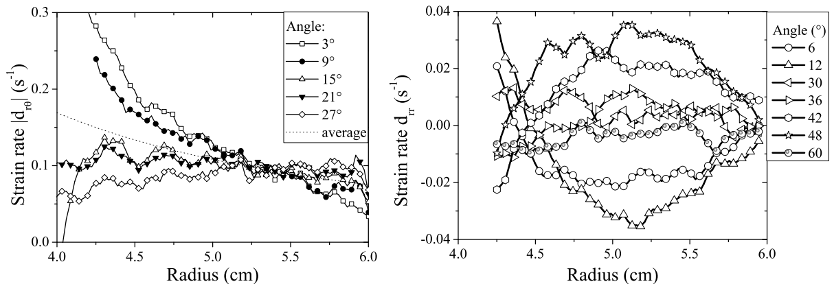
Figure 5: Strain rate profiles d_{r\theta}(r, \theta) (left) and d_{rr}(r, \theta) (right) vs. radius r for various angular positions \theta between two adjacent blades (from \theta = 0^\circ to \theta = 60^\circ ).
