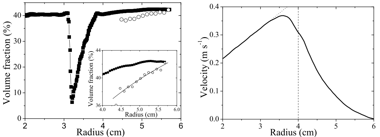
Figure 9: a) Steady-state volume fraction vs. radius at \Omega = 100 rpm in both the Couette geometry (empty circles) and the vane-in-cup geometry (squares). In the vane-in-cup geometry, the profile is performed in a 1 cm thick slice situated exactly between two adjacent blades (see Fig. 10b). The inset is a zoom; the line is a fit of the data measured in the Couette geometry to the Phillips et al. (1992) model with K_c/K_\mu = 0.42 . b) \theta -averaged orthoradial velocity profile \bar{V}_\theta(r) ; the dotted line is the theoretical rigid motion induced by the rotation of the vane tool; the dashed line shows the radius of the blades.
