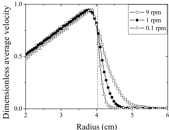
Figure 6: Dimensionless \theta -averaged velocity profile \bar{V}_\theta(r, \Omega)/\Omega R_i of a yield stress fluid (dense emulsion) in a 6-bladed vane-in-cup geometry for \Omega ranging from 0.1 to 9 rpm; the dashed line shows the radius of the blades; the dotted line is the theoretical profile for a rigid body rotation (for r < R_i ).
