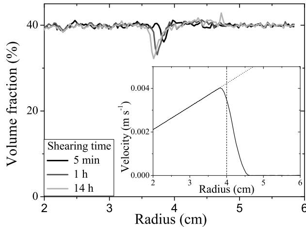
Figure 11: Volume fraction vs. radius at \Omega = 1 rpm measured in the vane-in-cup geometry after different times of shear: 5min, 1h, 14h. The material is homogeneous at the beginning of shear. The inset presents the \theta -averaged orthoradial velocity profile \bar{V}_\theta(r) measured in the first stages of shear; the dotted line is the theoretical rigid motion induced by the rotation of the vane tool; the dashed line shows the radius of the blades.
