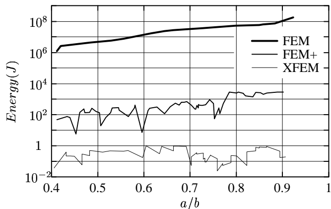
Figure 2. Cumulated energy out of balance
