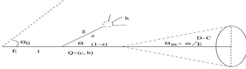
Figure 1: Parton splitting in the process Q \rightarrow Qg : a dead cone with opening angle \Theta_m is schematically shown.
