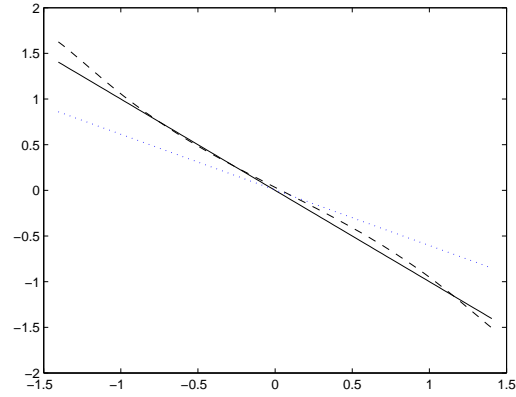
Figure 6: Ornstein-Uhlenbeck: estimation of b n = 10^4, \Delta = 1
