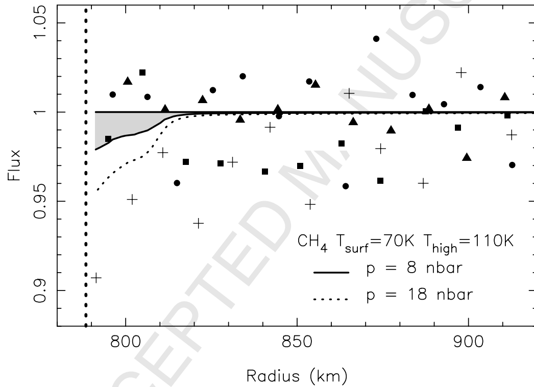
Fig. 16.— Same as Fig. 15, but for methane. The smooth solid line is the 1\text{-}\sigma upper limit for a heated \text{CH}_4 atmosphere with T = 70 \text{ K} at surface level and T = 110 \text{ K} above 20 \text{ km} , with a surface pressure of 8 \text{ nbar} . The shaded area shows the difference between this model and an airless model, while the dotted line shows the 3\text{-}\sigma upper limit ( p = 18 \text{ nbar} ) for comparison. See Table 5 and text for details.
