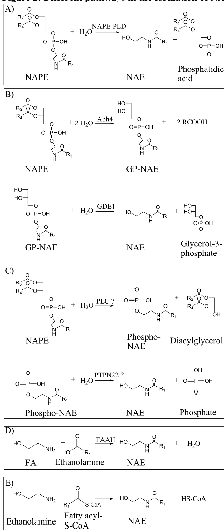
Figure 2: Different pathways in the formation of NAEs
