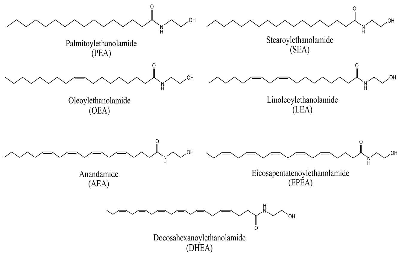
Figure 1: Structure of N -acylethanolamine
