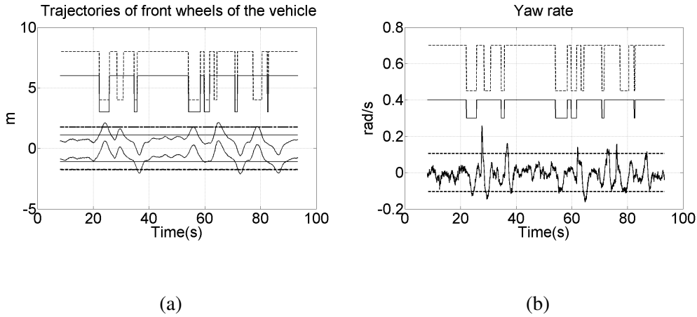
Fig. 12. (a) Trajectories of the front wheels (solid line), predefined lane strip \pm d = \pm 1.1m (solid line), lane border (dash-dot line), assistance activated for the first switching strategy on 3 (solid line), assistance activated for the second switching strategy on 4 (dashed line). (b) Yaw rate r (solid line), “normal driving” value r^N (dashed line), assistance activated for the first switching strategy on 0.3 (solid line), assistance activated for the second switching strategy on 0.45 (dashed line).
