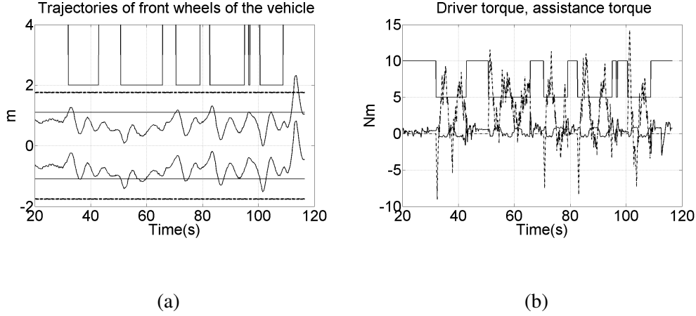
Fig. 6. (a) Trajectories of the front wheels (solid line), predefined lane strip \pm d = \pm 1.1m (solid line), computed driving lane strip \pm d_{ext} = \pm 1.76m (dashed line), lane borders at \pm 1.75m (dash-dot line, this coincides with the previous dashed line), assistance activated on 2 (first activation rules). (b) Driver's torque (solid line), assistance torque (dash-dot line), assistance activated on 5 (first activation rules).
