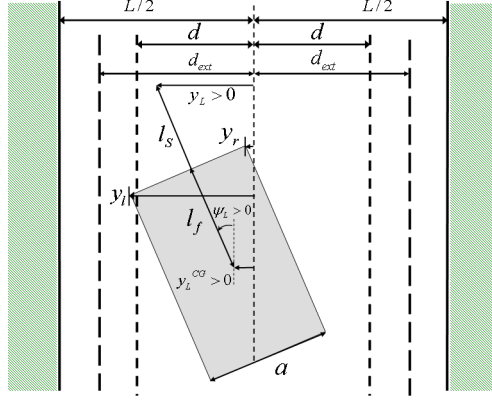
Fig. 2. Vehicle in the lane.
