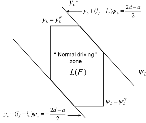
Fig. 3. “Normal driving” zone represented in a two-dimensional state space ((y_L, \psi_L)) .
