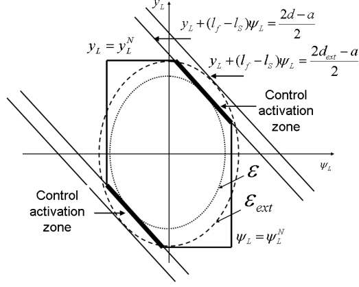
Fig. 4. The polyhedron L(\mathbf{F}) and the ellipsoids \mathcal{E} and \mathcal{E}_{ext} , represented in a two-dimensional state space (y_L, \psi_L) .
