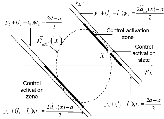
Fig. 7. Control activation for the new switching strategy.
