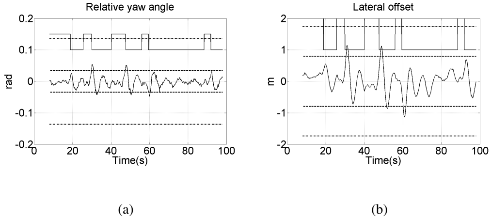
Fig. 10. (a) Relative yaw angle \psi_L (solid line), “normal driving” value \psi_L^N (dashed line), maximum computed bound \psi_L^M (dash-dot line), assistance activated on 0.1 (second activation rules). (b) Lateral offset y_L (solid line), “normal driving” value y_L^N (dashed line), maximum computed bound y_L^M (dash-dot line), assistance activated on 1 (second activation rules).
