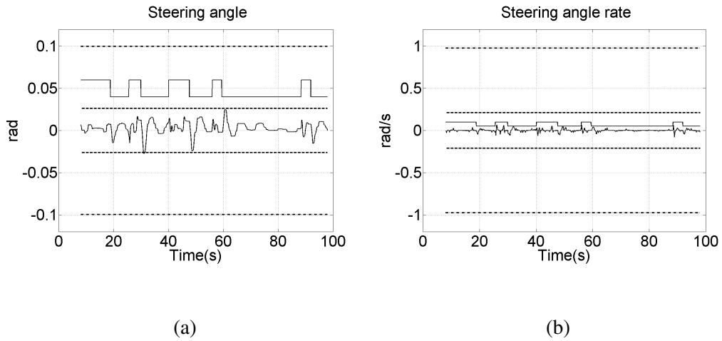
Fig. 11. (a) Steering angle \delta_f (solid line), “normal driving” value \delta_f^N (dashed line), maximum computed bound \delta_f^M (dash-dot line), assistance activated on 0.04 (second activation rules). (b) Steering angle rate \dot{\delta}_f (solid line), “normal driving” value \dot{\delta}_f^N (dashed line), maximum computed bound \dot{\delta}_f^M (dash-dot line), assistance activated on 0.05 (second activation rules).
