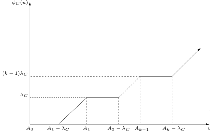
Figure 2: Function \phi_C .
