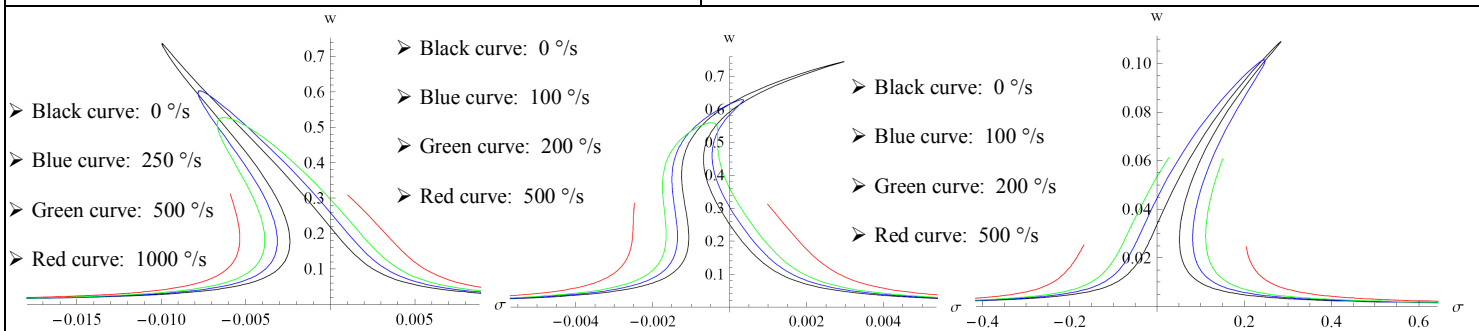
Fig.3.a: Softening behaviour
