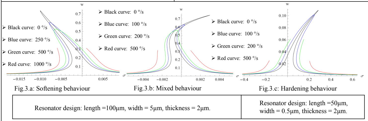
Fig.3: Predicted forced frequency responses for different angular rates of the resonant microgyroscope at a frequency equal to the resonator frequency with different kinds of behaviour. W_{\text{max}} is the normalized displacement with respect to the gap.
