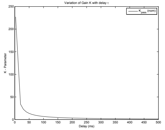
Fig. 2. Passivity Gain variation with delay
