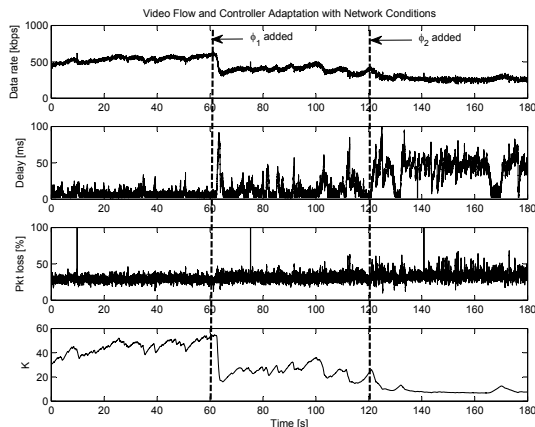
Fig. 9. QoS evaluation for Gain Adaptation
