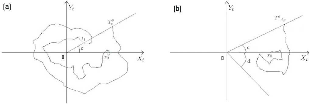
Figure 1: This figure presents the Exit times (a) T_c^\theta ( t_1 doesn't count because the angle is negative) and (b) T_{-d,c}^\theta for a planar BM starting from x_0 + i0 .
