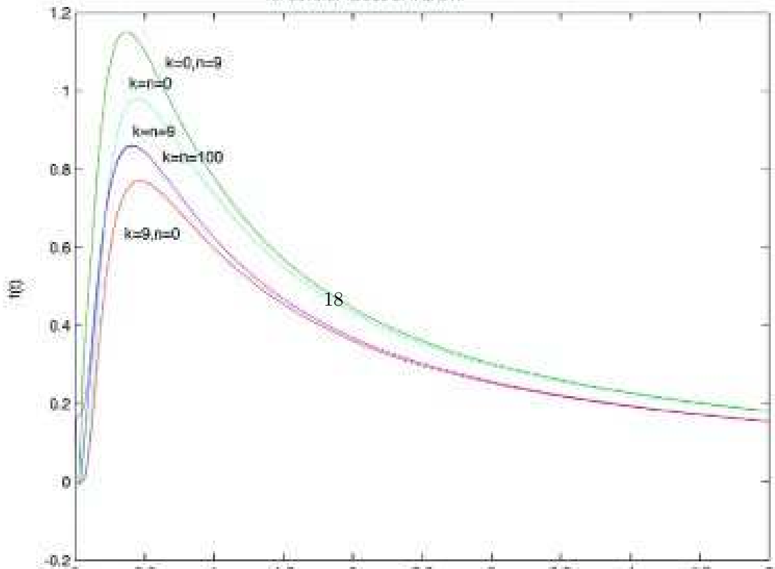
Figure 4: The diagram of f(t) with respect to the time t for several values of k and n .
