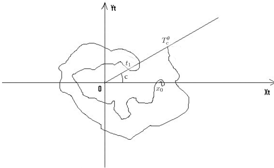
Figure 1: Diagram for T_c^\theta . The planar BM starts from x_0 + i0 . t_1 does not count because the angle is negative.
