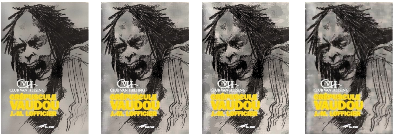
(a) Iterated TMR filter on EQ(u) .
