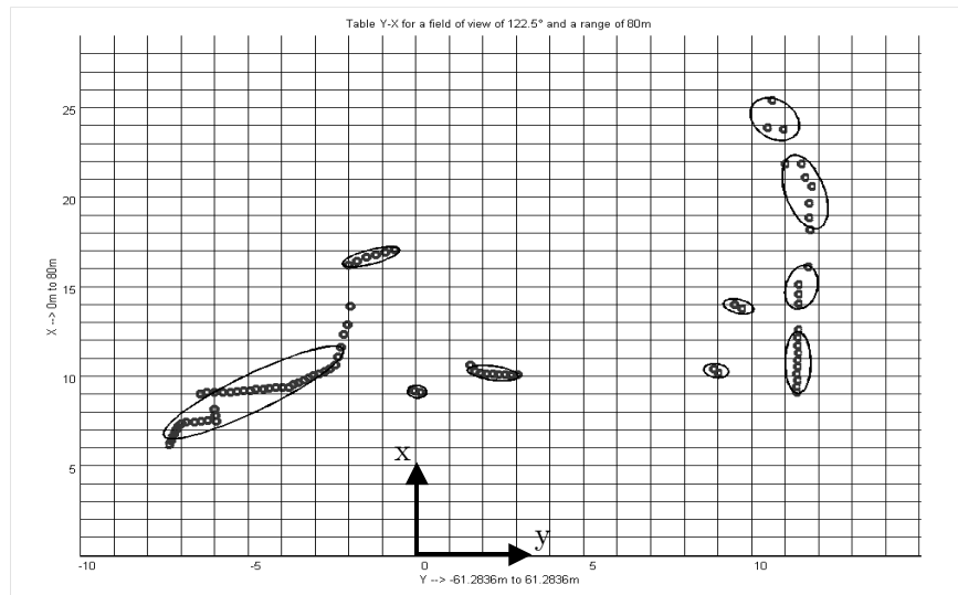
Fig. 4. Example of dynamic clustering (black ellipsoids) from laser scanner raw data (little circles).
