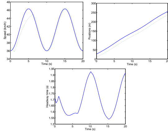
Fig. 4. Simulation of a car-following control - (-) leader (...) controlled vehicle - L=5m , h=1s
