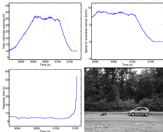
Fig. 8. Stop on obstacle - (-) leader (...) controlled vehicle - L=10m , h=3s
