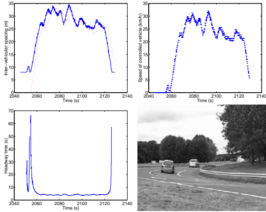
Fig. 7. Low speed car-following control by differential odometry - (-) leader (...) controlled vehicle - L=8m , h=3s
