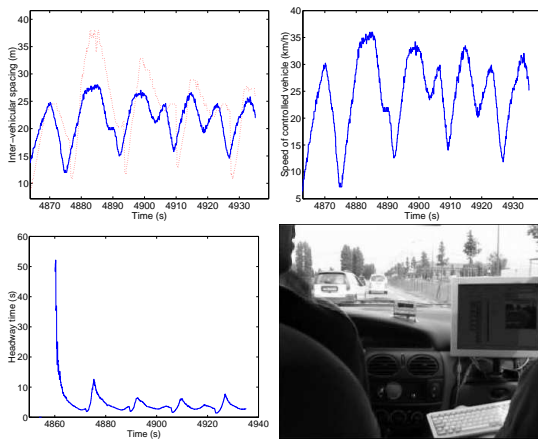
Fig. 11. Merging/overtaking influence - (-) leader (...) controlled vehicle - L=8m , h=2s
