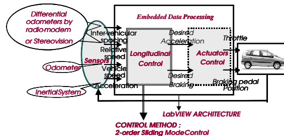
Fig. 6. Global system architecture
