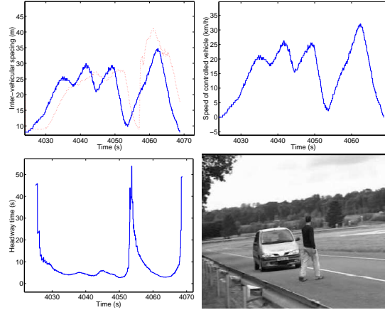
Fig. 9. Stop on pedestrian crossing by stereovision - (-) leader (...) controlled vehicle - L=8m , h=3s
