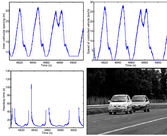
Fig. 10. Stopgo with stereovision - (-) leader (...) controlled vehicle - L=8m , h=3s
