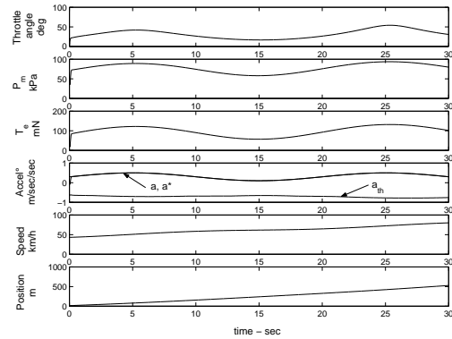
Fig. 3. Simulation for sinusoidal acceleration input
