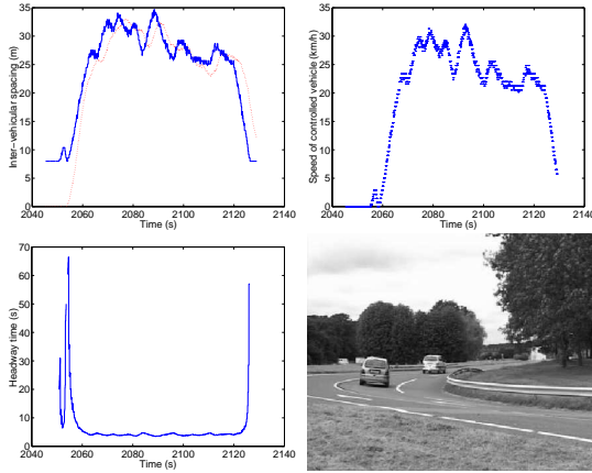
Fig. 7. Low speed car-following control by differential odometry - (-) leader (...) controlled vehicle - L=8m , h=3s
