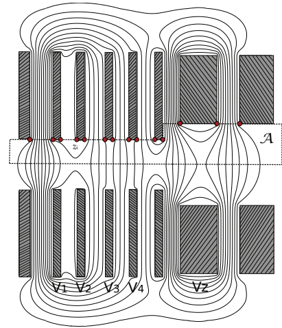
FIGURE 3: (Color online) A section of one side of the trap : the crosshatched areas are the electrodes, the continuous lines are the equipotentials, the domain \mathcal{A} is surrounded by a dashed border and the circled points represent the z_i points, which define our boundary conditions.
