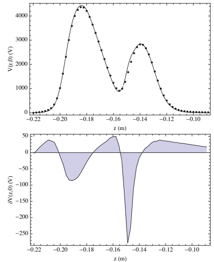
FIGURE 2: (Color online) The line represents the analytical function and the dots is the numerical solution achieved with the finite elements software COMSOL Multiphysics® (top). The difference between the two previous curves (bottom). In this case, we applied Bertram's method replacing R by a function of z . Even though the function is a polynomial going smoothly from R_z to R , we see that the error is large (-258V) near z = 0.15 where the transition occurs. Here \{V_1 = 4513 \text{ V}, V_2 = 4836 \text{ V}, V_3 = 3112 \text{ V}, V_4 = 1642 \text{ V}, V_z = ,3941 \text{ V}\} .
