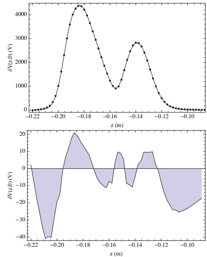
FIGURE 6: (Color online) The line represents the analytical function and the dots is the numerical solution (top). The difference between the two previous curves (bottom). We see that the error is around 1% and its smooth repartition shows that it does not arises from the varying radius. This difference is the consequence of the approximation we used to fix V(R, z) between the electrodes. Here \{V_1 = 4513 \text{ V}, V_2 = 4836 \text{ V}, V_3 = 3112 \text{ V}, V_4 = 1642 \text{ V}, V_z = 3941 \text{ V}\} .
