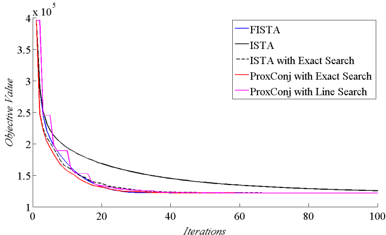
Figure 2: Comparaision of different algorithms on a synthesis problem.
