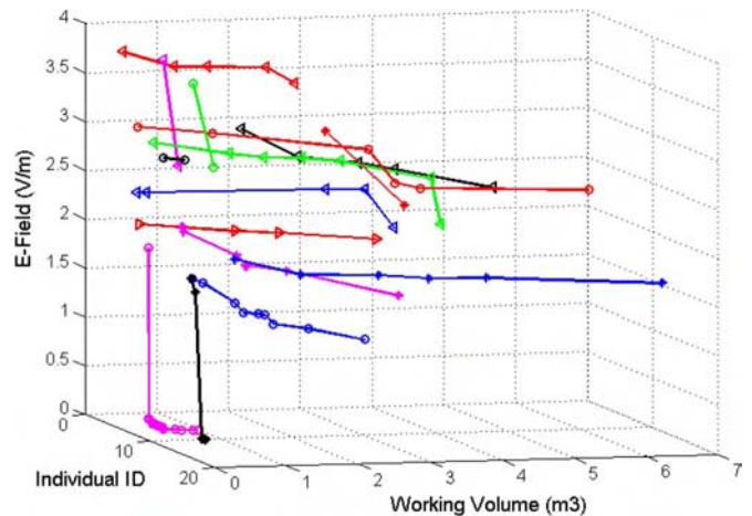
Fig. 8. Resulting Pareto front for the first generation from optimization process.
