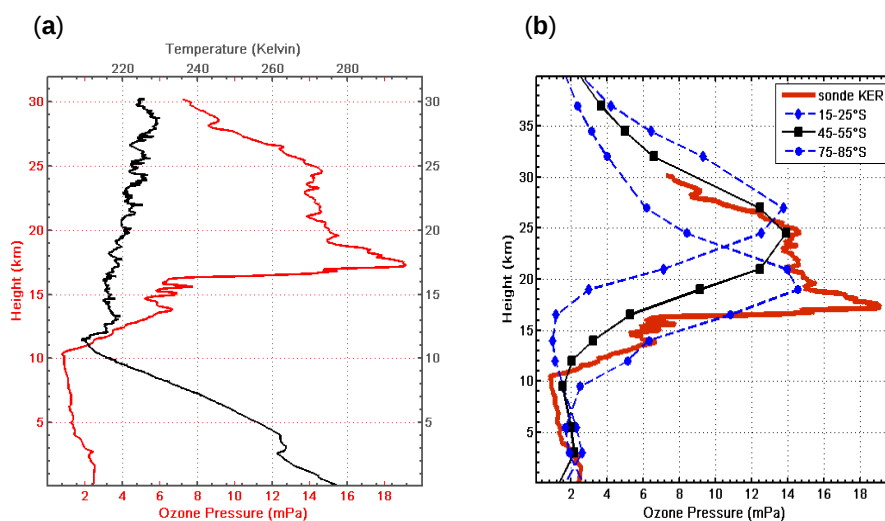
Fig. 1. (a) Vertical profiles of temperature (black line, in Kelvin) and ozone (red line, in mPa) obtained over Kerguelen ( 49.4^{\circ} S, 70.3^{\circ} E) as measured by the first balloon-sonde with ozone ECC sensor on 16 April 2008. (b) Same ozone profile (partial pressure in mPa, red continuous thick line) superimposed together with climatological ozone profiles derived from Fortuin & Kelder ozone climatology for three separate latitudinal belts ( 15^{\circ} – 25^{\circ} ; 45^{\circ} – 55^{\circ} and 75^{\circ} – 85^{\circ} ) of the Southern Hemisphere (see legend).
