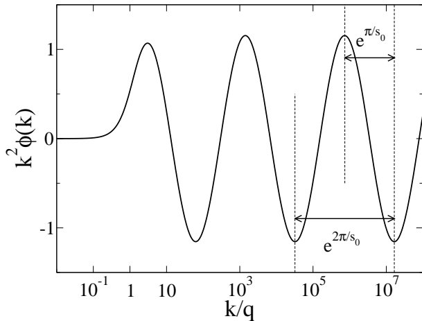
FIG. 1: Shape of the expression of k^2\phi(k) in Eq. (122) plotted in a semi-log plot as a function of k/q .
