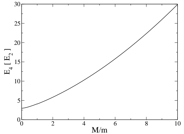
FIG. 7: Ground state branch for the three bosons of mass M interacting with one impurity of mass m in 2D as a function of the mass ratio.
