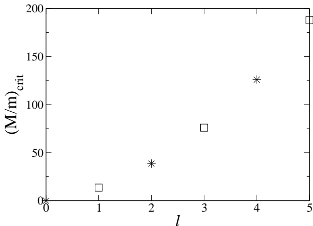
FIG. 5: Critical mass ratio (\frac{M}{m})_{\text{crit}}^l for the threshold of apparition of an Efimov spectrum in each partial wave l of Eq. (142).
