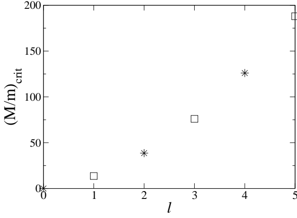
FIG. 5: Critical mass ratio (\frac{M}{m})_{\text{crit}} for the threshold of apparition of an Efimov spectrum in each partial wave l of Eq. (142).
