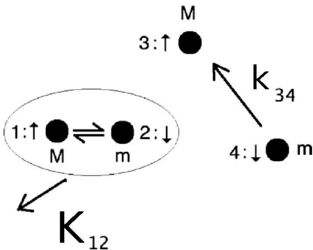
FIG. 6: Schematic representation of the momentum coordinates used for the source amplitude associated with the contact condition between particles 1 and 2 for a system of fermions with two-mass components.
