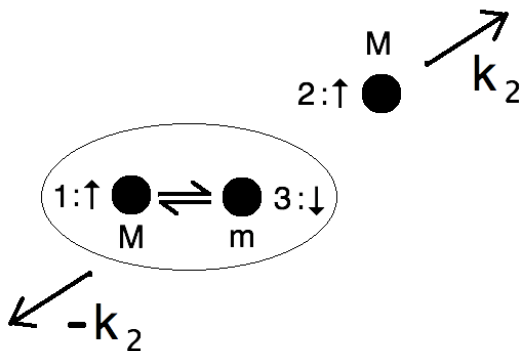
FIG. 4: Schematic representation of the momentum coordinates used for the source amplitude associated with the contact condition between particles 1 and 3.
