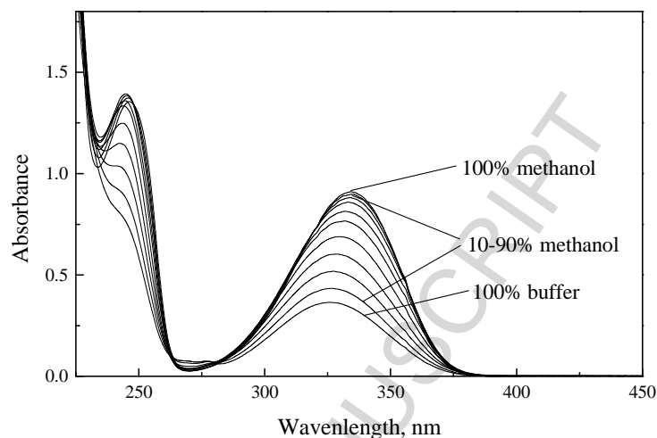
Figure 2. Absorption spectra of 1.0 \cdot 10^{-4} M solutions of anthranilic acid in different methanol – buffer mixtures (0 - 100% (v/v)).
