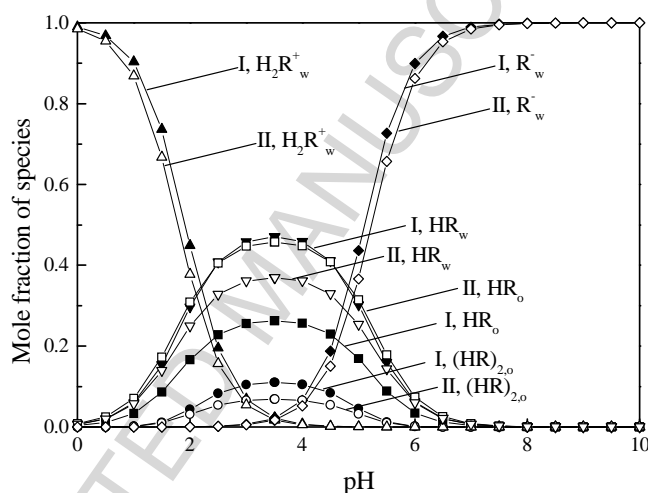
Figure 8. pH dependence of mole fraction of anthranilic acid species in the two-phase systems: organic solvent (I ethylbenzene, II nitrobenzene) – aqueous solution.
