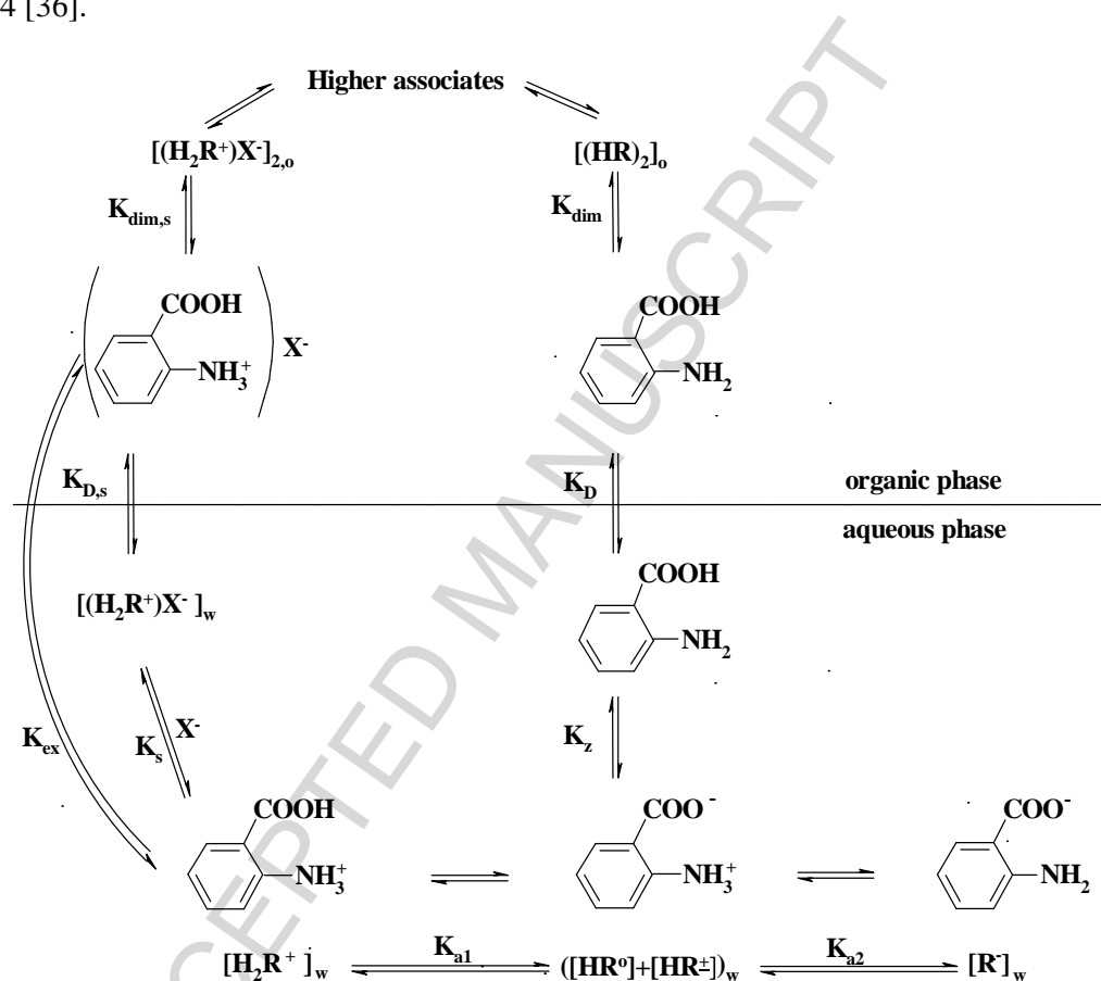
Figure 4. Reaction scheme for amino acid in two-phase system: organic solvent – aqueous solution (KCl, I = 0.1 ).
