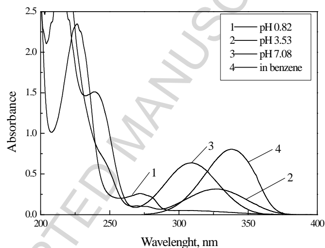
Figure 6. UV spectra of anthranilic acid in benzene and aqueous phase at different pH values.
