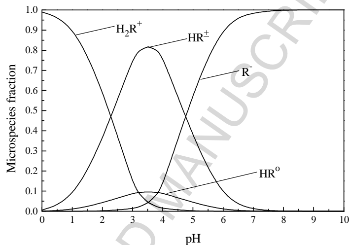
Figure 3. Microspeciation diagram of anthranilic acid.
