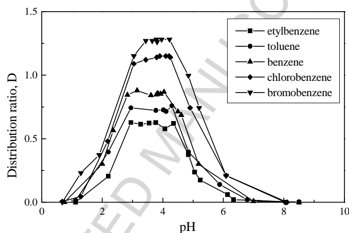
Figure 5. The values of the distribution ratio D of anthranilic acid in the two-phase system: organic solvent (ethylbenzene, toluene, benzene, chlorobenzene, bromobenzene) – aqueous solution as a function of the aqueous phase pH.
